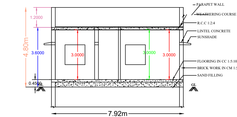
SECTION AB
