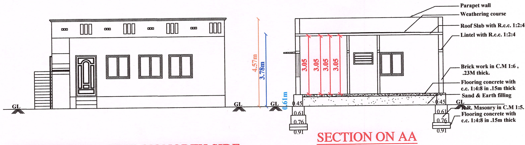
ELEVATION FACING ON NORTH SIDE
