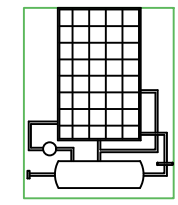
SOLAR SYSTEM
