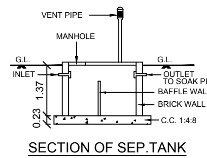
SECTION OF SEP.TANK
