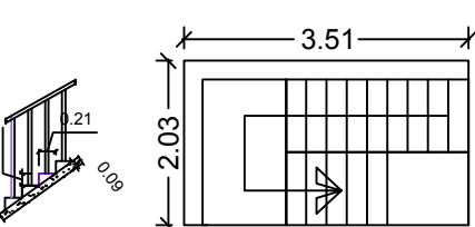
STAIRCASE DETAILS
