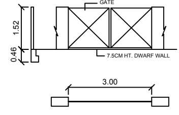
COMPOUND WALL WITH DWARF WALL DETAILS
