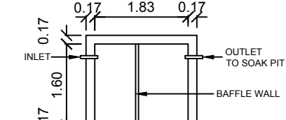
PLAN SEPTIC TANK
