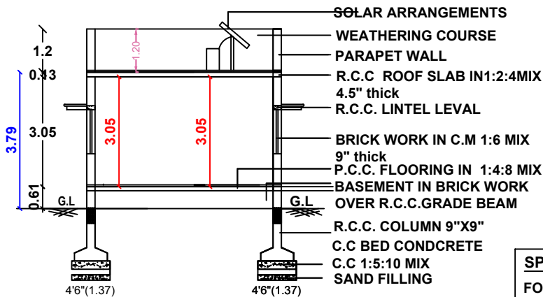
SECTION " AB "
