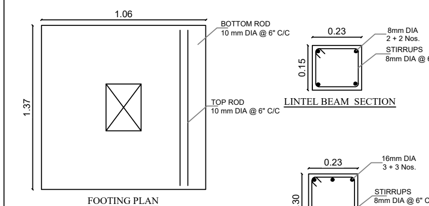
FOOTING PLAN
