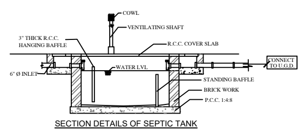
SECTION DETAILS OF SEPTIC TANK
