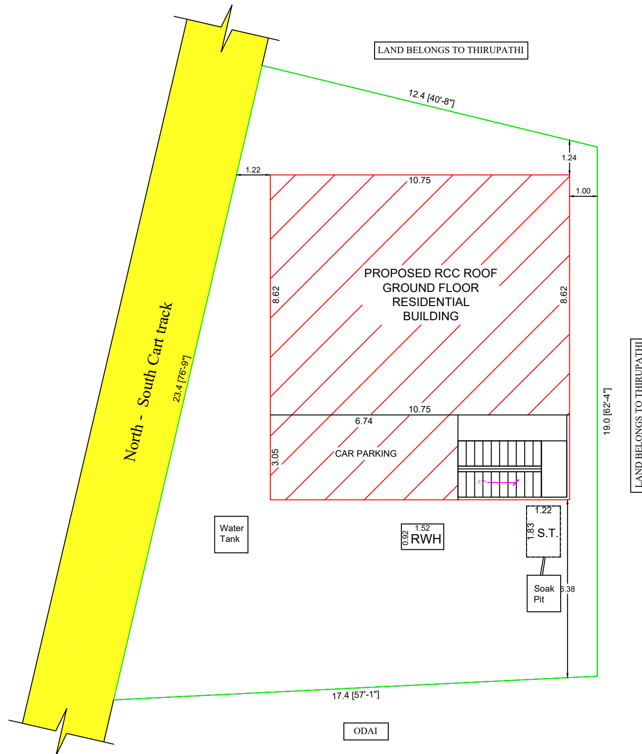
SITE PLAN
