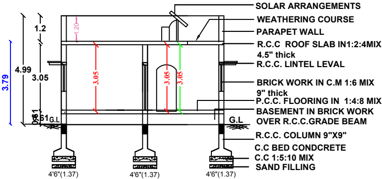
SECTION " AB "
