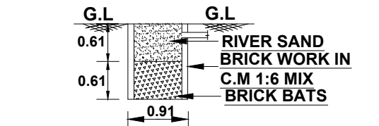
. SECTION ON RAIN WATER COLLECTION TUB .
