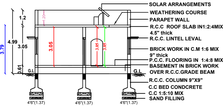
SECTION " AB "
