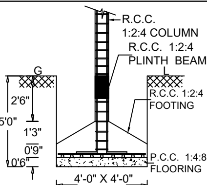
FOUNDATION DETAIL
