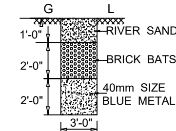
RAIN WATER PERCOLATION PIT (NTS)
