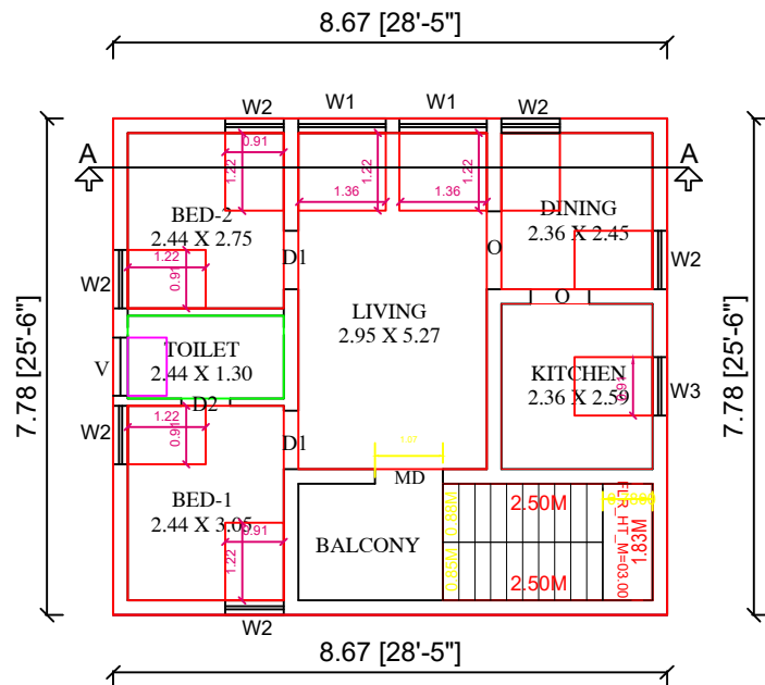
PROPOSED FIRST FLOOR PLAN (ONLINE APPROVAL)
