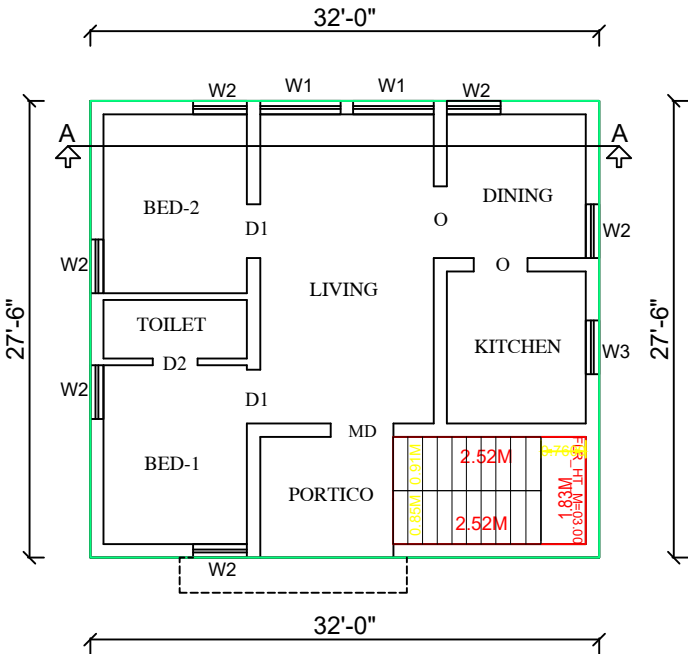
EXISTING GROUND FLOOR PLAN (MANUAL APPROVAL)
