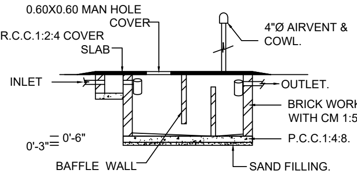
SEPTIC TANK DETAIL
