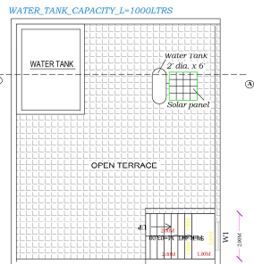
Proposed Terrace Floor Plan
