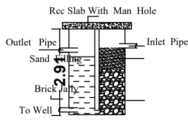
RWHTank Details
