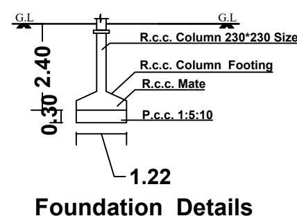
Foundation Details
