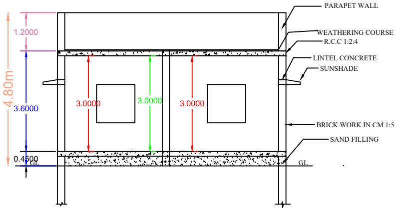
SECTION AB
