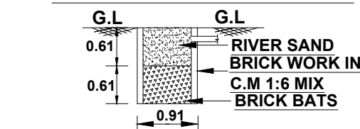
. SECTION ON RAIN WATER COLLECTION TUB .
