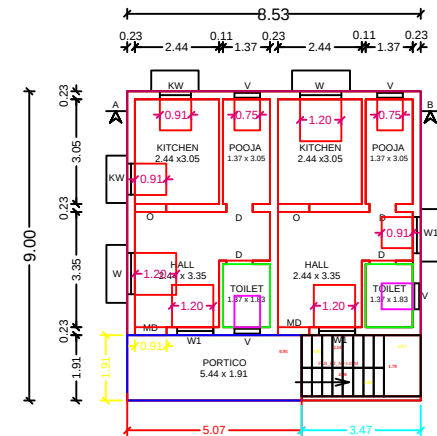
GROUND FLOOR PLAN (NORTH FACING)
