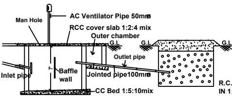
SECTION FOR SEPTIC TANK AND D.T (NOT TO SCALE)
