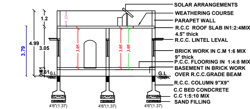
SECTION " AB "
