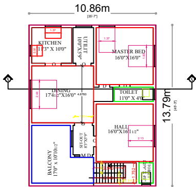
PROPOSED FRIST FLOOR PLAN
