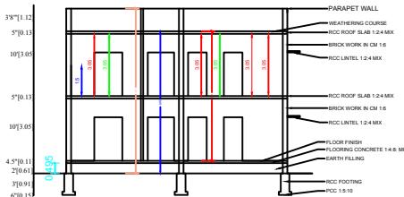
SECTION AB
