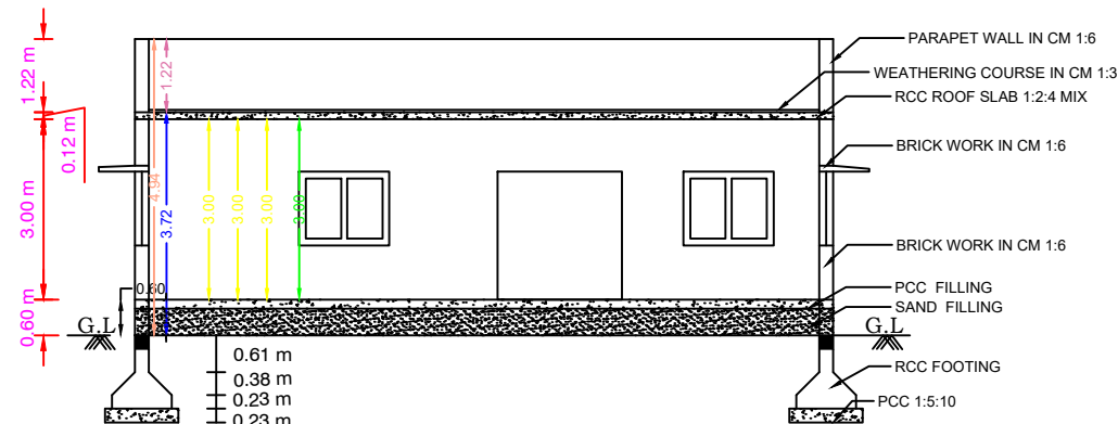
SECTION ON KA
