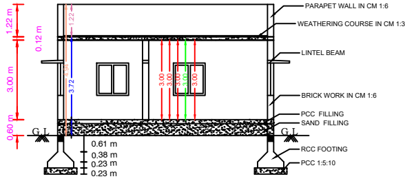
SECTION ON KA
