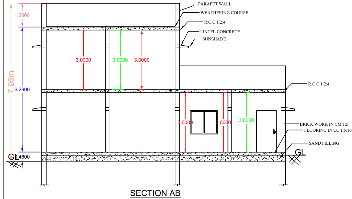
SECTION AB
