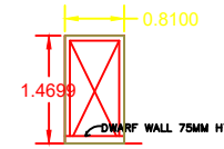
WICKET GATE
