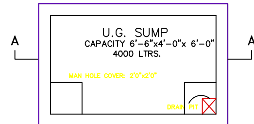
SUMP DETAIL SCALE 1"=4'-0"
