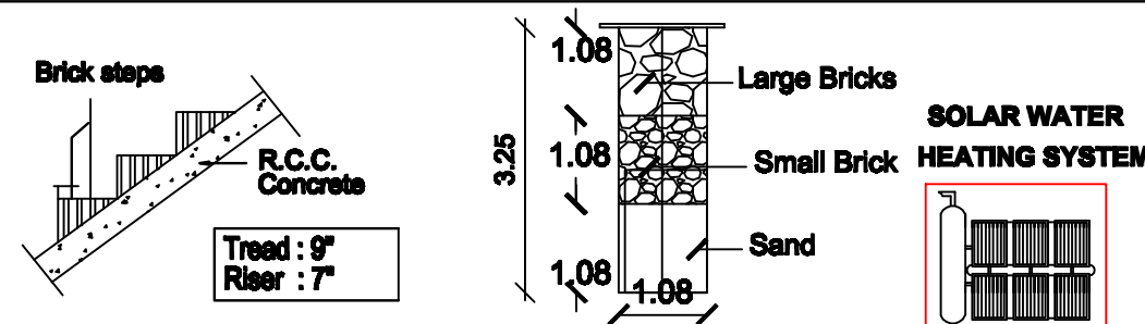
STAIRCASE DETAILS
