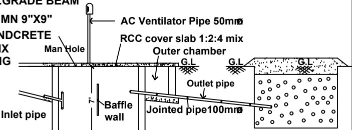
SECTION FOR SEPTIC TANK AND D.T (NOT TO SCALE)
