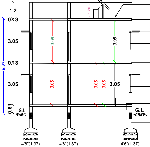
SECTION " AB "
