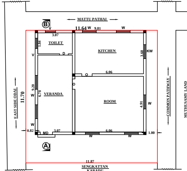
. GROUND PLAN .
