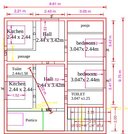
PROP.SECOND FLOOR PLAN
