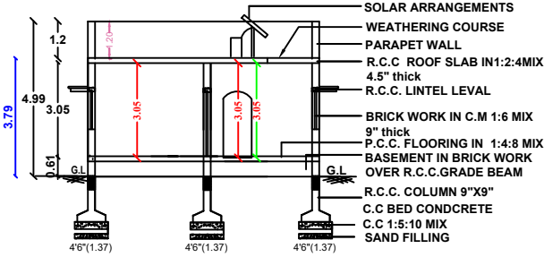
SECTION " AB "
