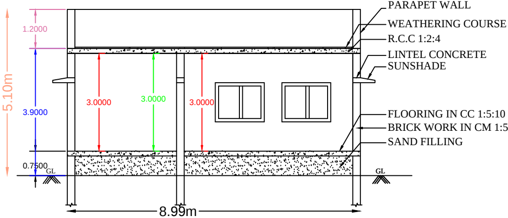
SECTION AB
