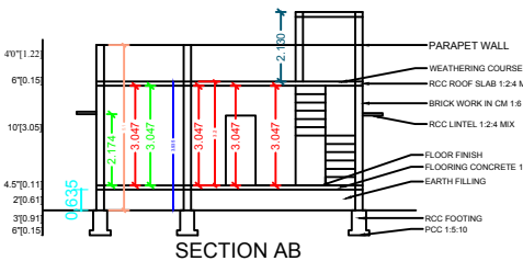
SECTION AB
