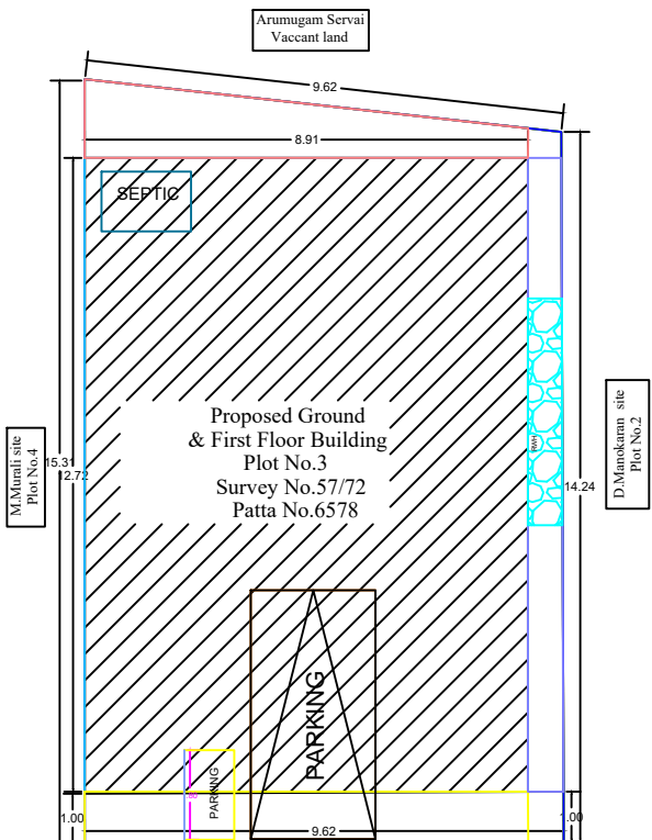
KEY PLAN
