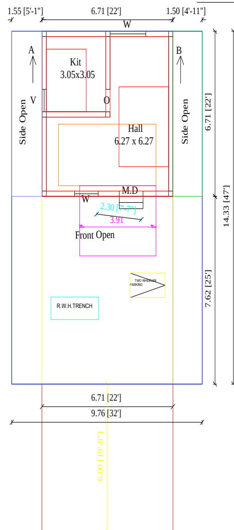
Pro.Ground Floor
