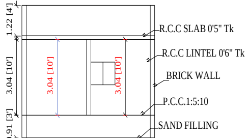
section on"AB"
