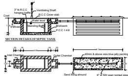
DETAILS OF SEPTIC TANK & DISPERSION TRENCH
