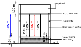
SECTION-"S'R"
