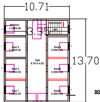
Block 1 Ground Floor Plan
