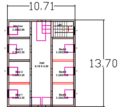
Block 1 First Floor Plan
