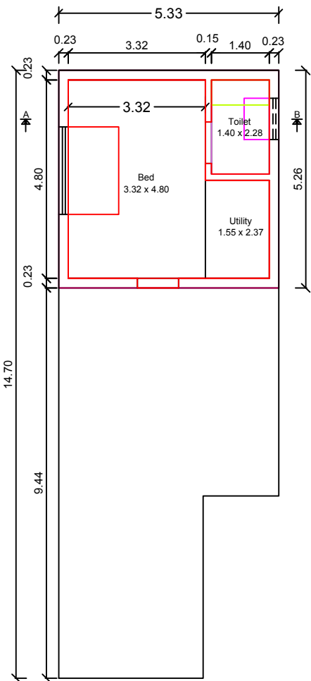
PRO.FIRST FLOOR PLAN
