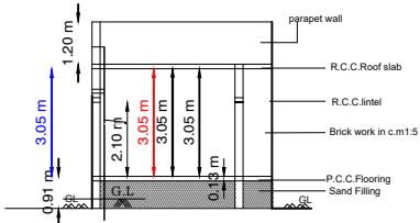
SECTION-"SR"
