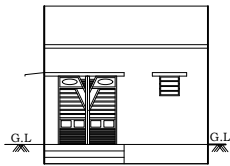
FRONT ELEVATION
