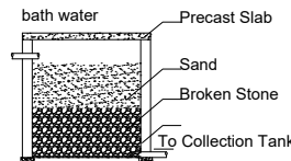
Section of Filter Unit
