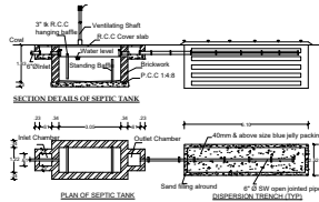
DETAILS OF SEPTIC TANK & DISPERSION TRENCH
