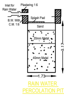
RAIN WATER PERCOLATION PIT
