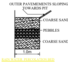
RAIN WATER PERCOLATION PIT
