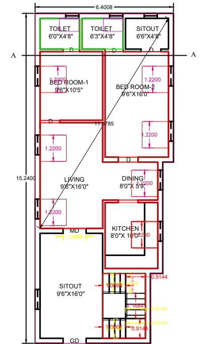
GROUND FLOOR PLAN [SOUTH FACING]
