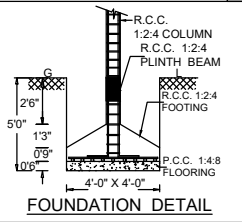
FOUNDATION DETAIL
