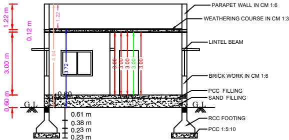
SECTION OF KA
