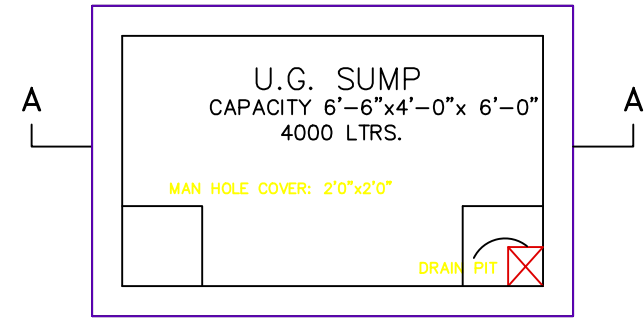
SUMP DETAIL SCALE 1"=4'-0"
