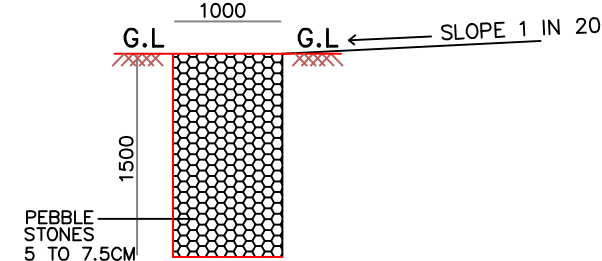
SECTION OF PEBBLE TRENCH SCALE : 1: = 100
