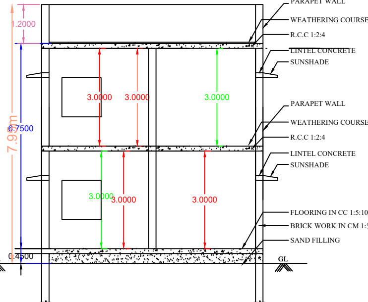
SECTION AB
