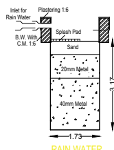
RAIN WATER PERCOLATION PIT
