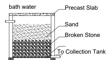
Section of Filter Unit
