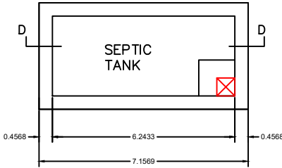
PLAN OF SEPTIC TANK SCALE: 1"=2'0"
