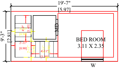
PROPOSED FIRST FLOOR PLAN
