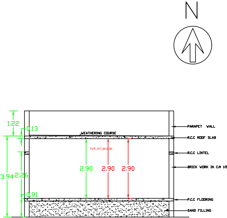
SECTION
