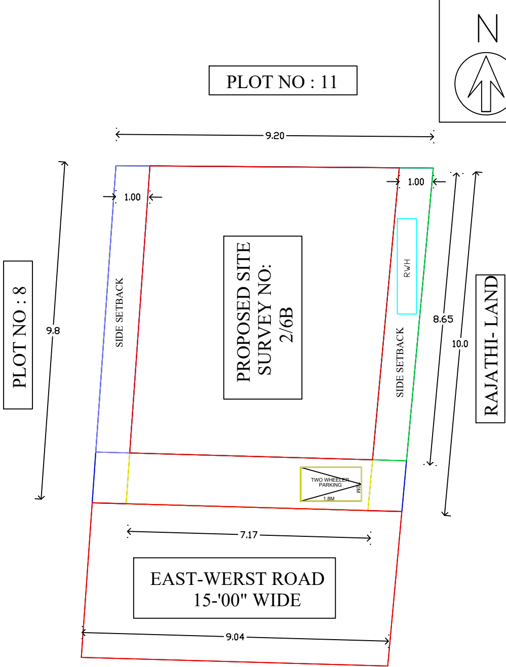
SITE PLAN (NOT FOR SCALE)
