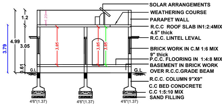
SECTION " AB "
