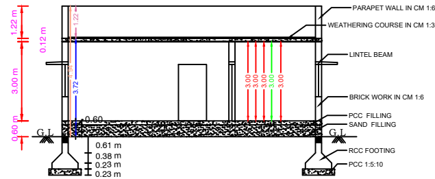
SECTION ON KA
