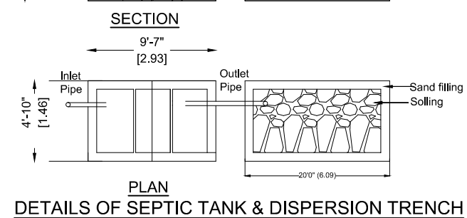
DETAILS OF SEPTIC TANK & DISPERSION TRENCH
