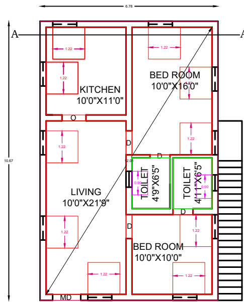
GROUND FLOOR PLAN [NORTH FACING]
