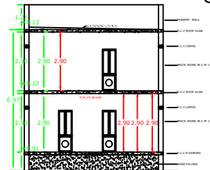
SECTION ON K-S
