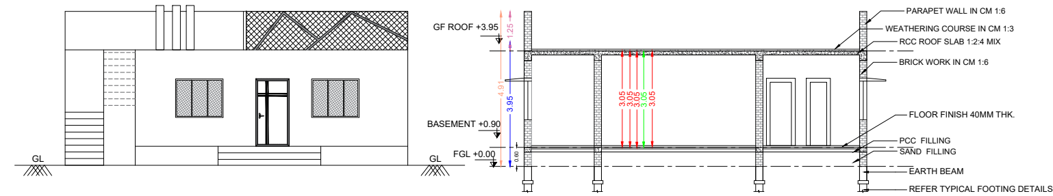
FRONT ELEVATION
