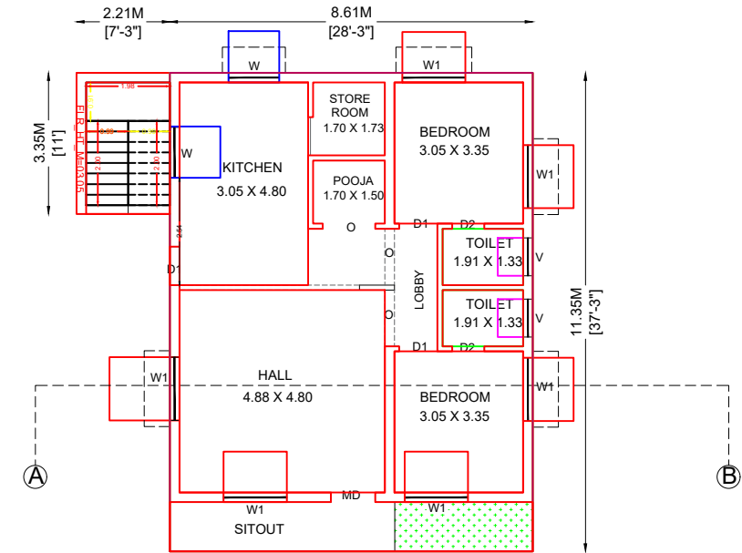
PROPOSED GROUND FLOOR PLAN (NORTH FACING)
