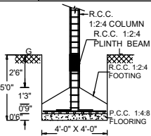
FOUNDATION DETAIL
