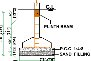
DETAILS OF COLUMN FOOTING FOUNDATION
