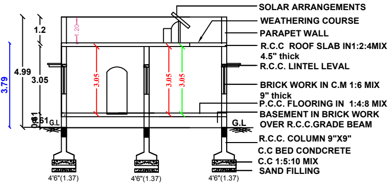
SECTION " AB "
