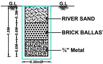
RAIN WATER HARVESTING SYSTEM
