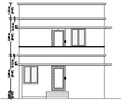
FRONT ELEVATION
