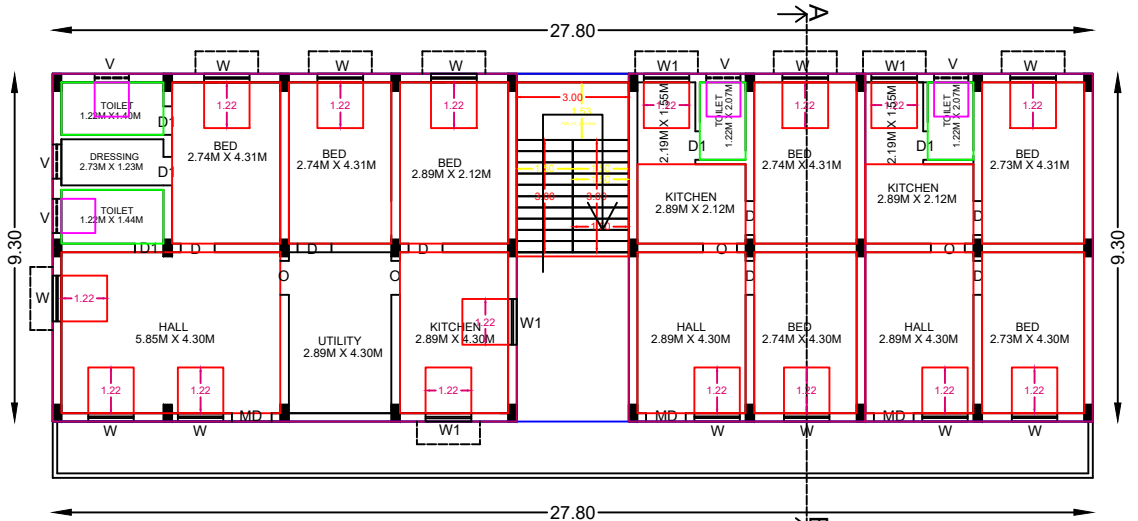
TYPICAL FIRST & SECOND FLOOR PLAN
