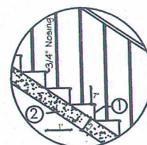
STAIRCASE SECTION
