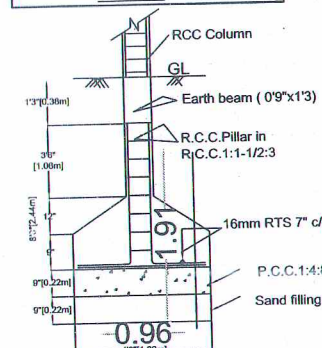
FOUNDATION DETAILS
